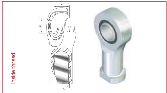
Rod end, steel / PTFE with inside thread
